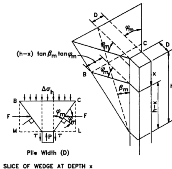
Figure 2-7: Basic strain wedge theory model in a uniform soil (Ashour et al., 1998)
